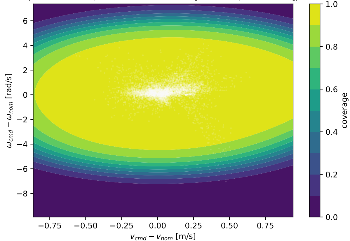
Residual coverage vs command offset (0 = off / OOD; state fixed at mean [0.59 m/s, 0.27 rad/s])
